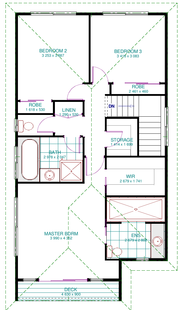
Upper level = 88 sq m
